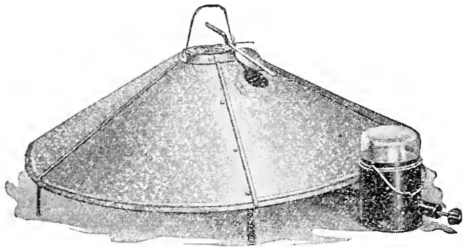
Leonard Bluepoint Oil Burning Brooder
